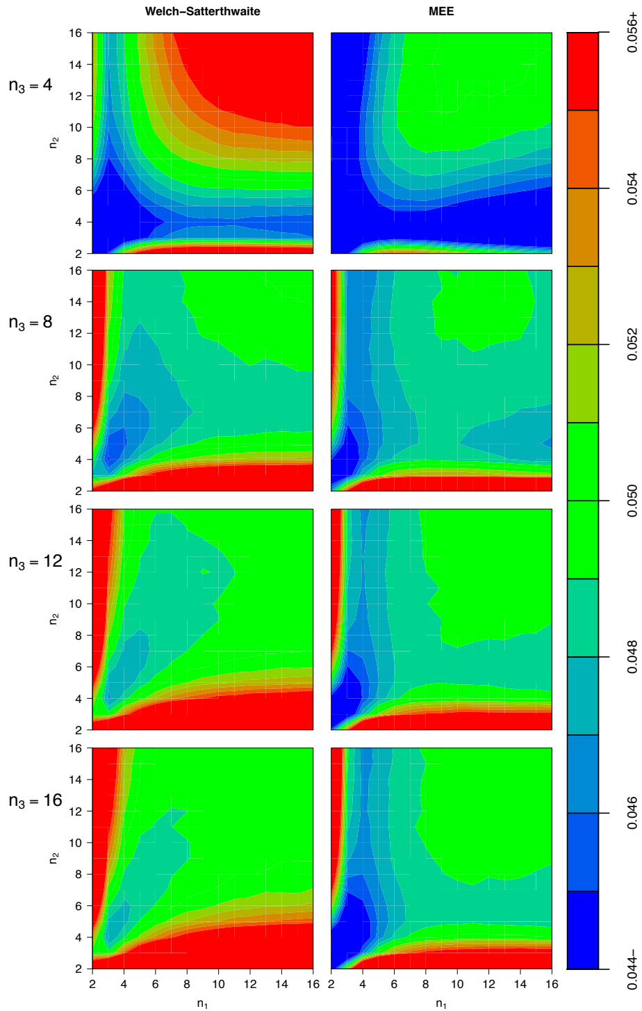
FIGURE 10. Filled contour plots of test level estimates for Welch-Satterthwaite (left column) and MEE (right column) as a function of n_1 , n_2 , and n_3 at the \alpha = .05 level of significance. \sigma_1^2 = 2 , \sigma_2^2 = 4 , and \sigma_3^2 = 1 for all the plots, while the rows correspond to n_3 = 4, 8, 12 , and 16 , respectively. Each combination is replicated b = 10^7 times.
