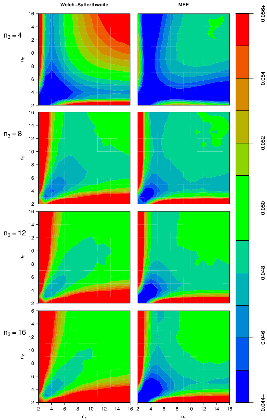
FIGURE 13. Filled contour plots of test level estimates for Welch-Satterthwaite (left column) and MEE (right column) as a function of n_1 , n_2 , and n_3 at the \alpha = .05 level of significance. \sigma_1^2 = 4 , \sigma_2^2 = 4 , and \sigma_3^2 = 1 for all the plots, while the rows correspond to n_3 = 4, 8, 12 , and 16 , respectively. Each combination is replicated b = 10^7 times.
