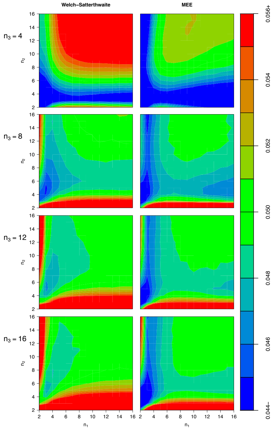
FIGURE 7. Filled contour plots of test level estimates for Welch-Satterthwaite (left column) and MEE (right column) as a function of n_1 , n_2 , and n_3 at the \alpha = .05 level of significance. \sigma_1^2 = 1 , \sigma_2^2 = 3 , and \sigma_3^2 = 1 for all the plots, while the rows correspond to n_3 = 4, 8, 12 , and 16 , respectively. Each combination is replicated b = 10^7 times.
