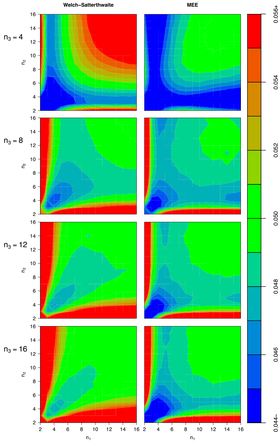
FIGURE 11. Filled contour plots of test level estimates for Welch-Satterthwaite (left column) and MEE (right column) as a function of n_1 , n_2 , and n_3 at the \alpha = .05 level of significance. \sigma_1^2 = 3 , \sigma_2^2 = 3 , and \sigma_3^2 = 1 for all the plots, while the rows correspond to n_3 = 4, 8, 12 , and 16 , respectively. Each combination is replicated b = 10^7 times.
