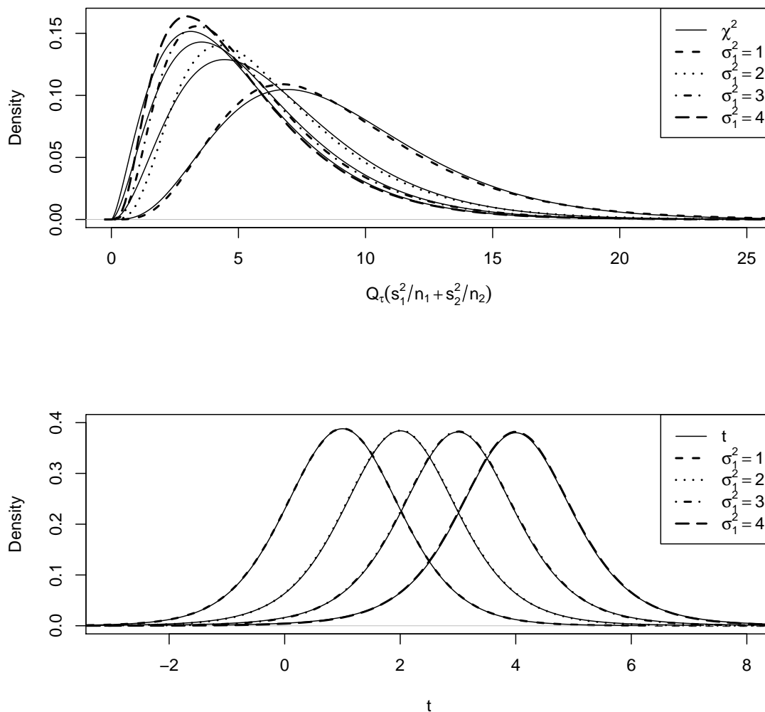
FIGURE 2. The upper panel shows the empirical density estimates for Q_\tau(s_1^2/n_1 + s_2^2/n_2) as various dashed outlines where n_1 = 5 , n_2 = 8 , \sigma_2^2 = 1 , and \sigma_1^2 = 1, 2, 3 , or 4 as indicated in the legend. The solid lines indicate the respective \chi^2 density approximations. The lower panel shows empirical density estimates for t = (\bar{x}_1 - \bar{x}_2) / \sqrt{s_1^2/n_1 + s_2^2/n_2} using the same configurations as the upper panel with approximating t -distribution densities overlaid as solid lines artificially recentered at 1, 2, 3, and 4, respectively. The tuning parameter \tau in each case was determined by Eq. (??) resulting in the degrees of freedom being calculated as 8.91, 6.45, 5.55, and 5.12, respectively. Each density estimate is based on b = 10^7 replications.
