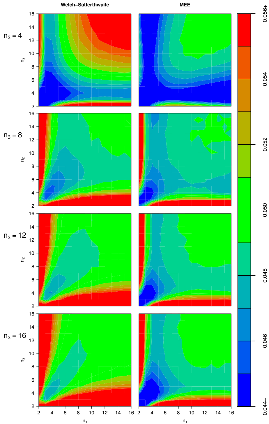
FIGURE 12. Filled contour plots of test level estimates for Welch-Satterthwaite (left column) and MEE (right column) as a function of n_1 , n_2 , and n_3 at the \alpha = .05 level of significance. \sigma_1^2 = 3 , \sigma_2^2 = 4 , and \sigma_3^2 = 1 for all the plots, while the rows correspond to n_3 = 4, 8, 12 , and 16 , respectively. Each combination is replicated b = 10^7 times.
