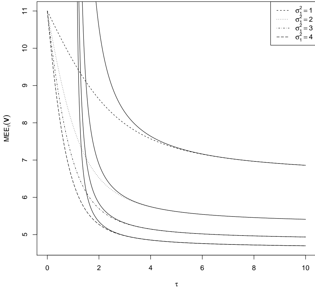
FIGURE 1. Plot of MEE_{\tau}[\mathbf{V}] as a function of \tau with \mathbf{V} as defined in Eq. (??), n_1 = 5 , n_2 = 8 , and \sigma_2^2 = 1 . The legend indicates the four different curves that correspond with \sigma_1^2 = 1, 2, 3 , and 4 , while the solid curves are the respective native scale approximations of MEE_{\tau}[\mathbf{V}] given by Eq. (??).
