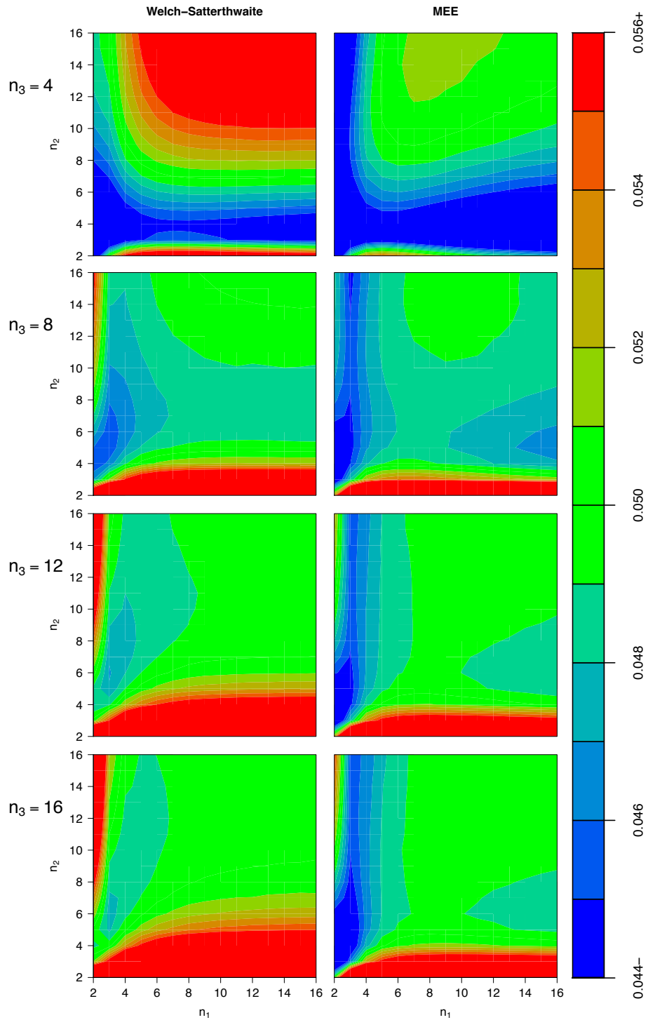
FIGURE 4. Filled contour plots of test level estimates for Welch-Satterthwaite (left column) and MEE (right column) as a function of n_1 , n_2 , and n_3 at the \alpha = .05 level of significance. \sigma_1^2 = 1 , \sigma_2^2 = 4 , and \sigma_3^2 = 1 for all the plots, while the rows correspond to n_3 = 4, 8, 12 , and 16 , respectively. Each combination is replicated b = 10^8 times.
