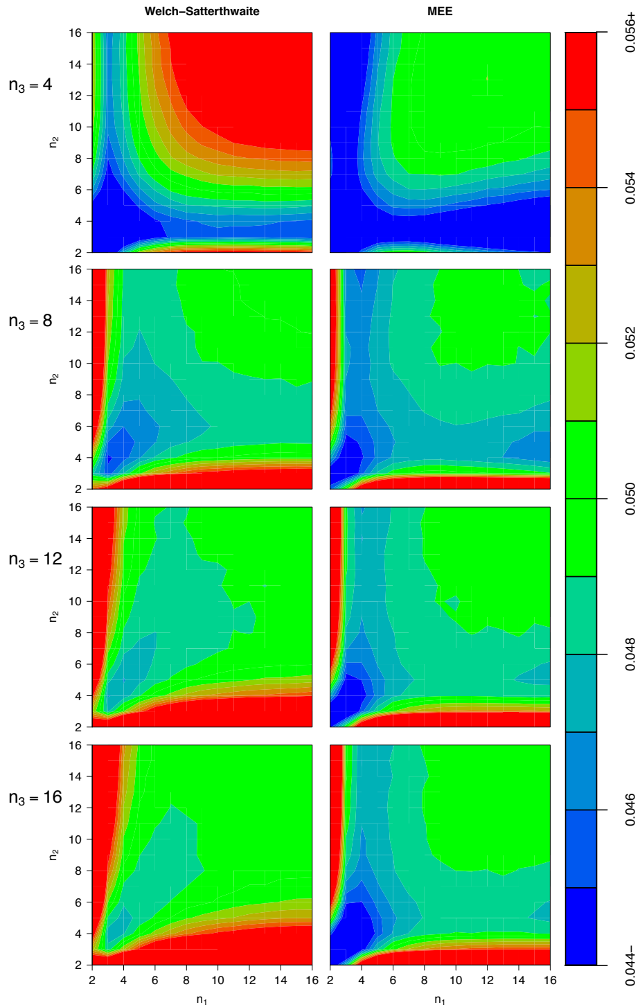
FIGURE 9. Filled contour plots of test level estimates for Welch-Satterthwaite (left column) and MEE (right column) as a function of n_1 , n_2 , and n_3 at the \alpha = .05 level of significance. \sigma_1^2 = 2 , \sigma_2^2 = 3 , and \sigma_3^2 = 1 for all the plots, while the rows correspond to n_3 = 4, 8, 12 , and 16 , respectively. Each combination is replicated b = 10^7 times.
