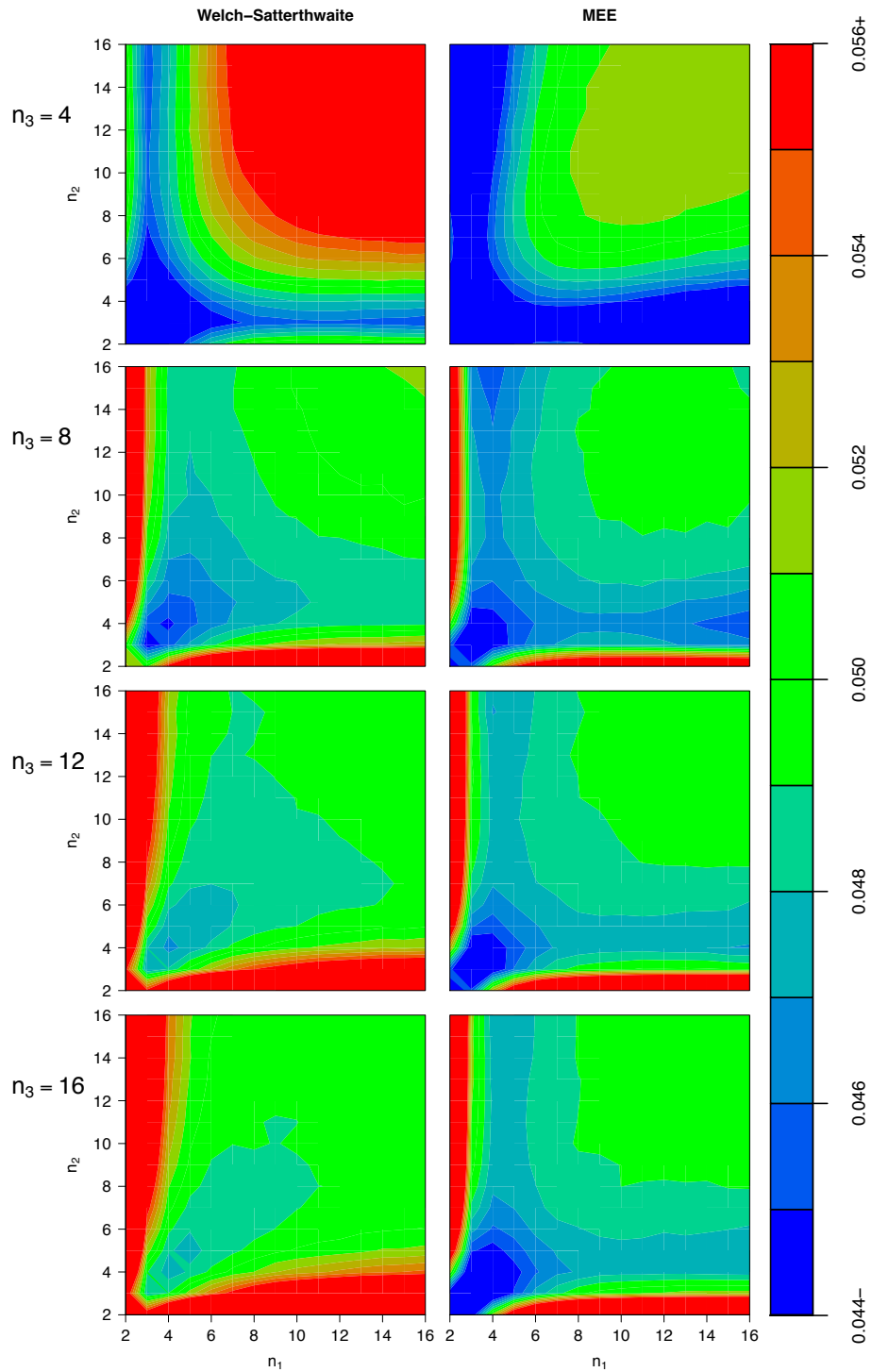
FIGURE 8. Filled contour plots of test level estimates for Welch-Satterthwaite (left column) and MEE (right column) as a function of n_1 , n_2 , and n_3 at the \alpha = .05 level of significance. \sigma_1^2 = 2 , \sigma_2^2 = 2 , and \sigma_3^2 = 1 for all the plots, while the rows correspond to n_3 = 4, 8, 12 , and 16 , respectively. Each combination is replicated b = 10^7 times.
