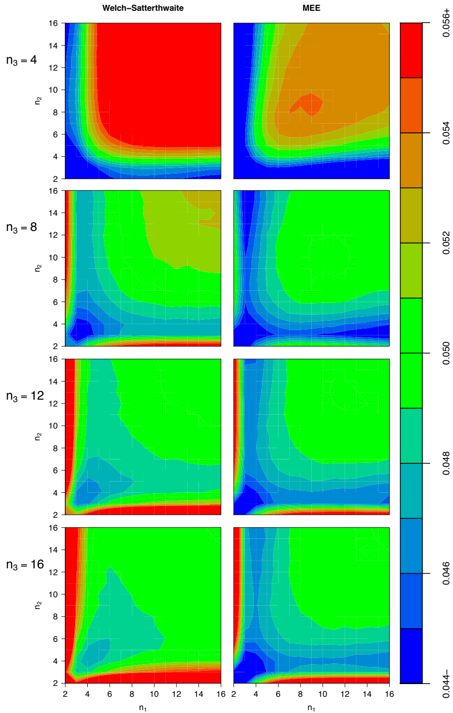
FIGURE 5. Filled contour plots of test level estimates for Welch-Satterthwaite (left column) and MEE (right column) as a function of n_1 , n_2 , and n_3 at the \alpha = .05 level of significance. \sigma_1^2 = 1 , \sigma_2^2 = 1 , and \sigma_3^2 = 1 for all the plots, while the rows correspond to n_3 = 4, 8, 12 , and 16 , respectively. Each combination is replicated b = 10^7 times.
