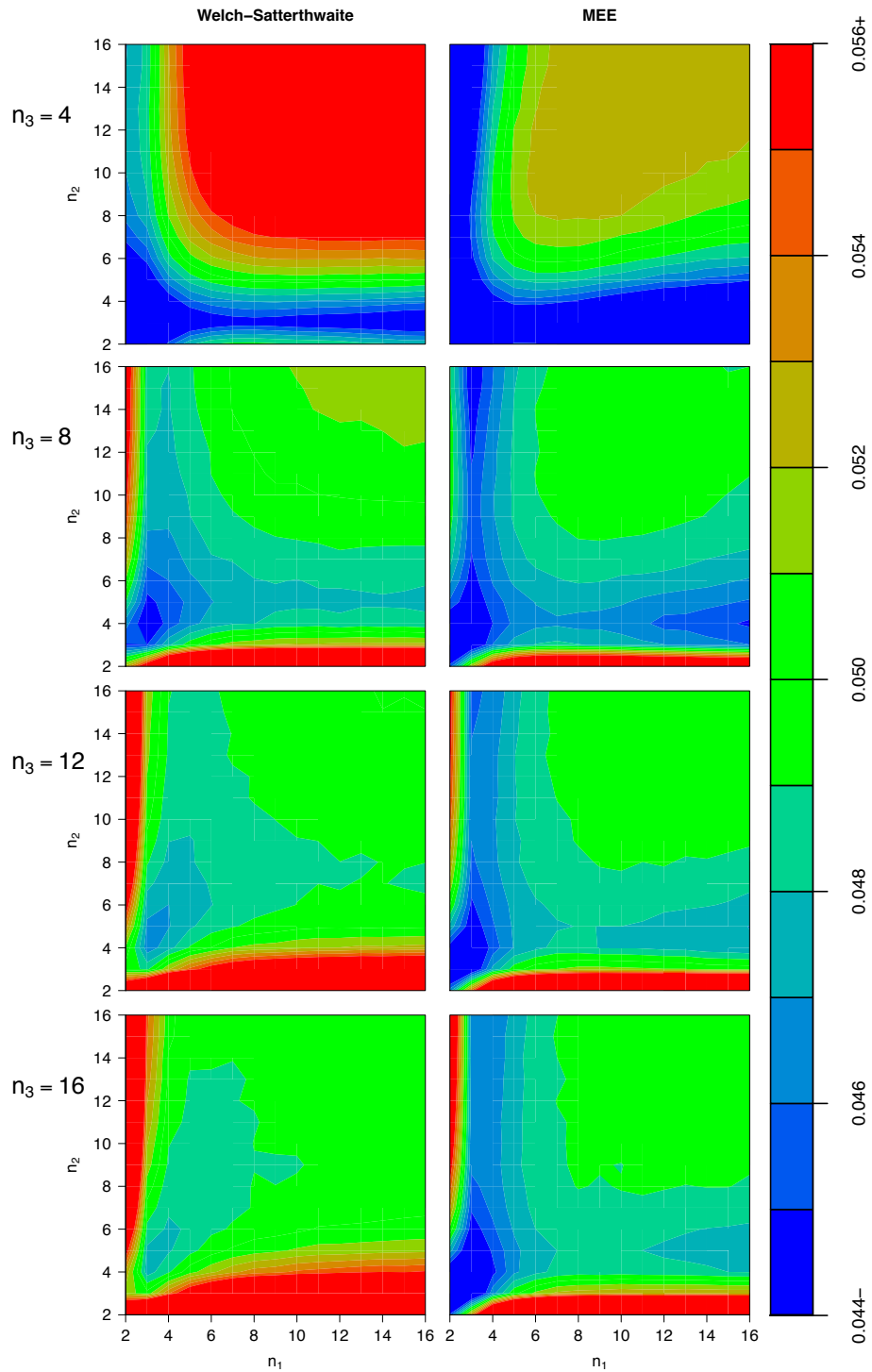
FIGURE 6. Filled contour plots of test level estimates for Welch-Satterthwaite (left column) and MEE (right column) as a function of n_1 , n_2 , and n_3 at the \alpha = .05 level of significance. \sigma_1^2 = 1 , \sigma_2^2 = 2 , and \sigma_3^2 = 1 for all the plots, while the rows correspond to n_3 = 4, 8, 12 , and 16 , respectively. Each combination is replicated b = 10^7 times.
